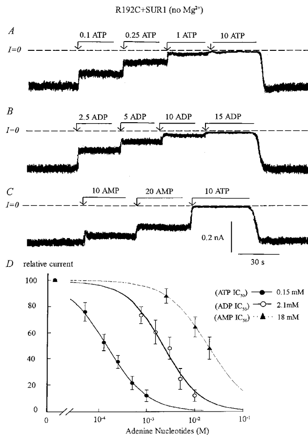
FIGURE 4 Adenine nucleotide sensitivity of the Kir6.2 mutant R192C+UR1. (A, B, and C) Inward currents measured in the absence of Mg^{2+} were suppressed by increasing concentrations of ATP, ADP, and AMP with the IC_{50} near 150 \mu M, 2 mM, and 18 mM, respectively. On average, ADP was 13-fold less potent and AMP 120-fold less potent than ATP at blocking the channel. Compared with wild-type channels, the ATP, AMP, and ADP sensitivity of the mutant decreased by ~10-fold. (D) Plot of channel ATP (●), ADP (○), and AMP (▲) sensitivity for Kir6.2+SUR1 in the absence of Mg^{2+} . Fit of the data points yielded k = 150 \mu M for ATP ( n = 3 ), k = 2.1 mM ( n = 3 ) for ADP, and k = 18 mM for AMP ( n = 3 ). The estimated Hill coefficients were close to unity for ATP and ADP data points. The AMP data were fitted using a Hill coefficient of 1.
