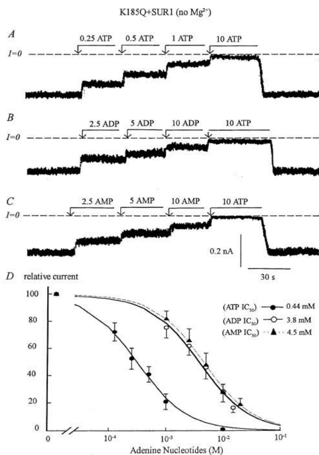
FIGURE 3 Adenine nucleotide sensitivity of the Kir6.2 mutant K185Q+SUR1. (A, B, and C) Inward currents measured in the absence of Mg^{2+} were progressively suppressed by increasing concentrations of ATP, ADP, and AMP with the IC_{50} near 440 \mu M, 3.8 mM, and 4.5 mM, respectively. On average ADP was eightfold less potent and AMP 10-fold less potent than ATP at blocking the channel. As compared to wild-type channels, the ATP and ADP sensitivity decreased by ~30-fold, while the AMP sensitivity was only 2.5-fold lower. (D) Plot of channel ATP (●), ADP (○), and AMP (▲) sensitivity for Kir6.2+SUR1 in the absence of Mg^{2+} . Fit of the data points yielded k = 0.44 mM for ATP ( n = 3 ), k = 3.8 mM ( n = 3 ) for ADP, and k = 4.5 mM for AMP ( n = 3 ). The three Hill coefficients were close to unity.
